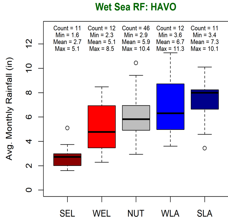
Figure 8. Boxplot of wet season monthly rainfall grouped by ENSO category. HAVO.
