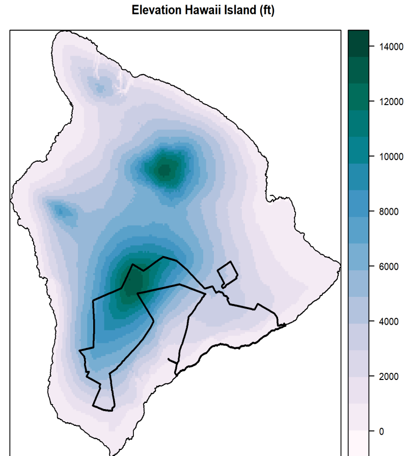
Figure 2. Elevation for the Island of Hawai'i Island with HAVO outlined in black. The maps shown in the following slides will be for the HAVO area only.
