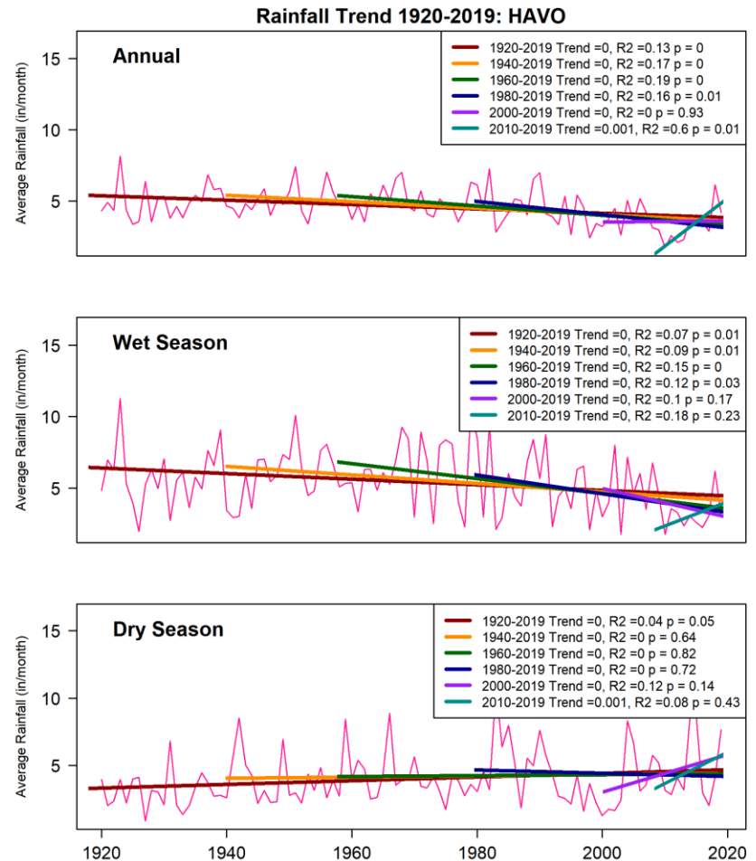
Figure 9. 100-year (1920-2019) rainfall time series at HAVO with linear trends calculated over six unique periods in the record; Trend is the slope ( inches per year); R^2 is the strength of the trend; p is a measure of the statistical significance.
