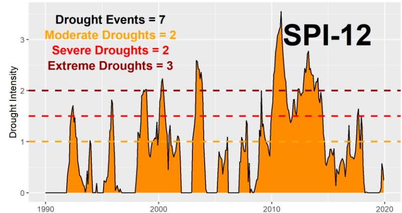
Figure 13. 30-year (1990-2019) SPI-12 time series (reversed axis) at Hawai'i Volcanoes National Park.
