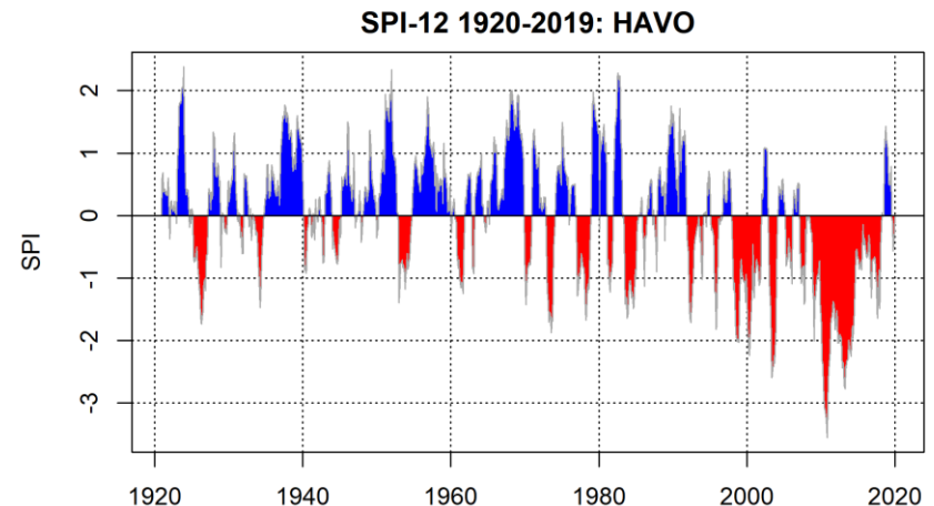
Figure 10. 100-year (1920-2019) SPI-12 time series at HAVO positive SPI (blue) indicate wet periods, negative SPI (red) indicate dry periods.
