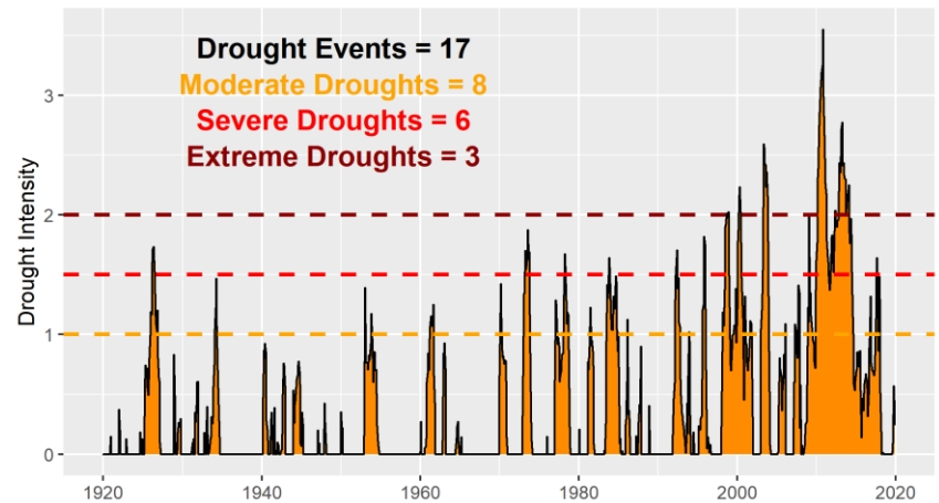
SPI-12 Drought Events 1920 -2019: HAVO
