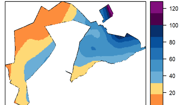
Figure 7. Dry and Wet season total rainfall at HAVO.
