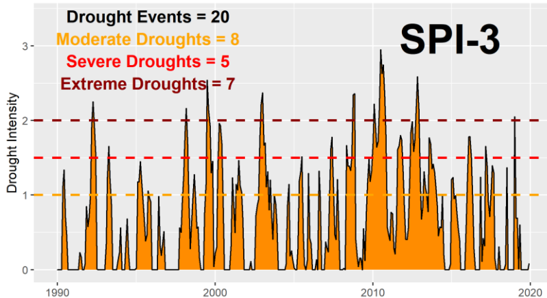
Figure 12. 30-year (1990-2019) SPI-3 time series (reversed axis) at Hawai'i Volcanoes National Park.
