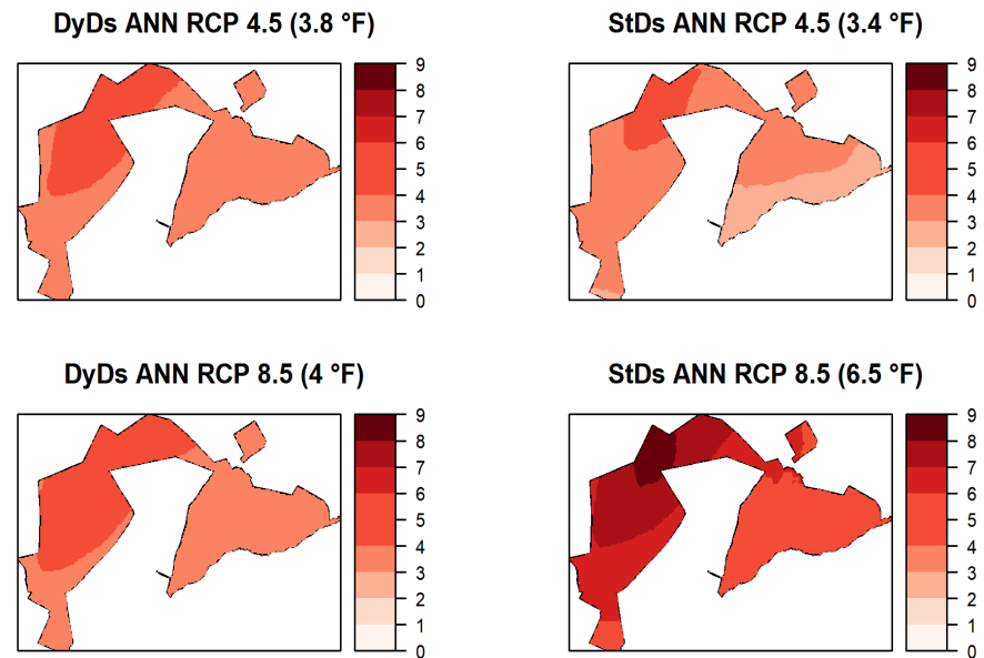
Figure 17. Downscaled projected change in mean temperature (Year 2100) at HAVO, Dynamical Downscaling (DyDs), Statistical Downscaling (StDs).
