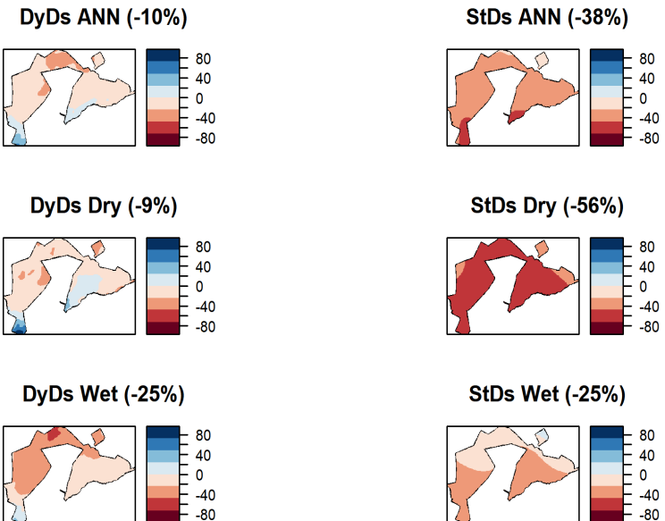
Figure 15. Downscaled future rainfall projections (% Change; (2100) at HAVO, Dynamical Downscaling (DyDS), Statistical Downscaling (StDs), for annual (ANN), dry season (DRY) and wet season (WET).
