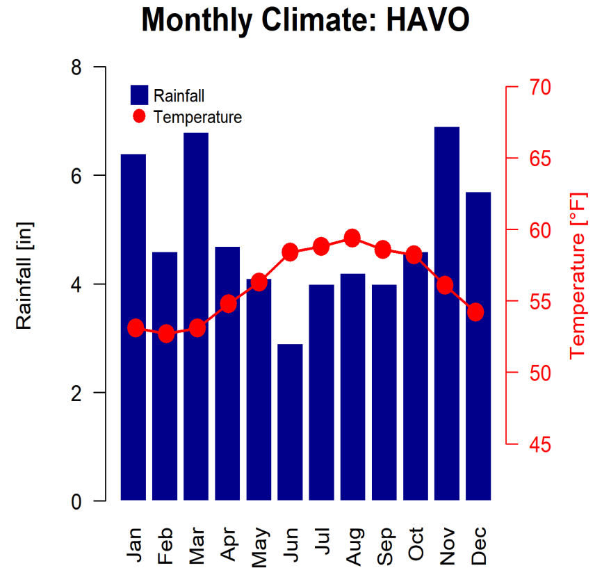
Figure 4. Mean monthly rainfall and temperature at HAVO.
